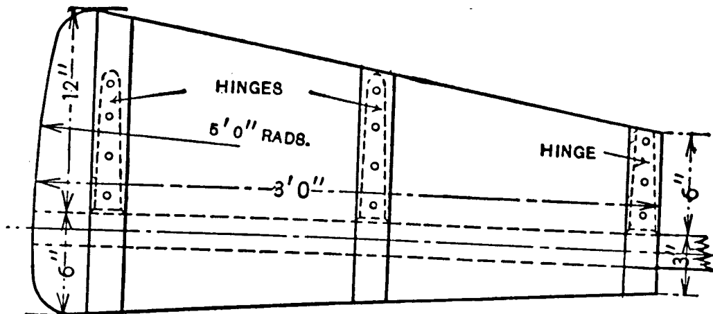
FIG. 56.—Outline of Sail for 10-foot Windmill.
